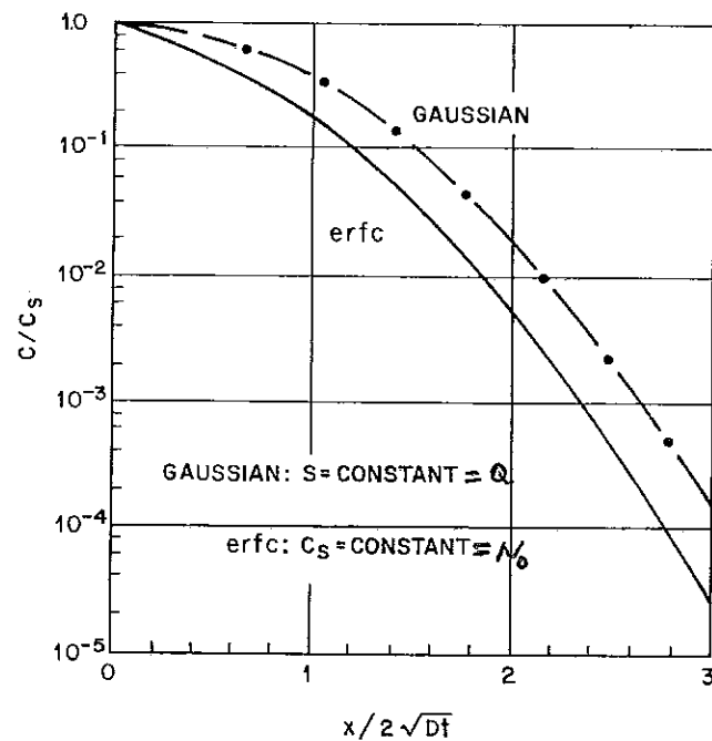
Fig. 5 Normalized concentration versus normalized distance for the erfc and the Gaussian function.
